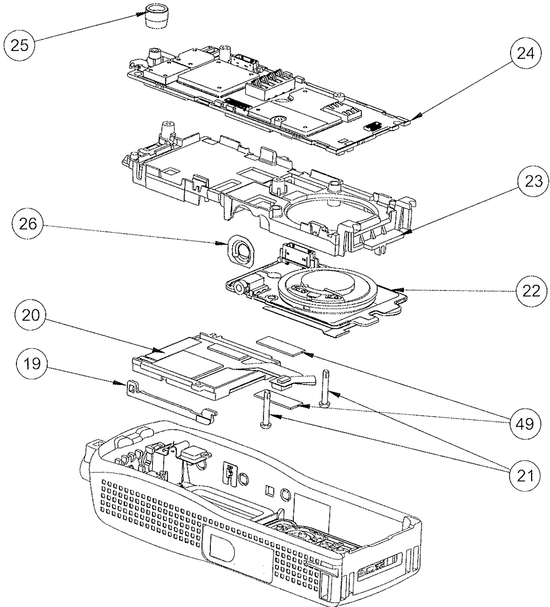
Figure 23 MTP850 — Exploded View 2
