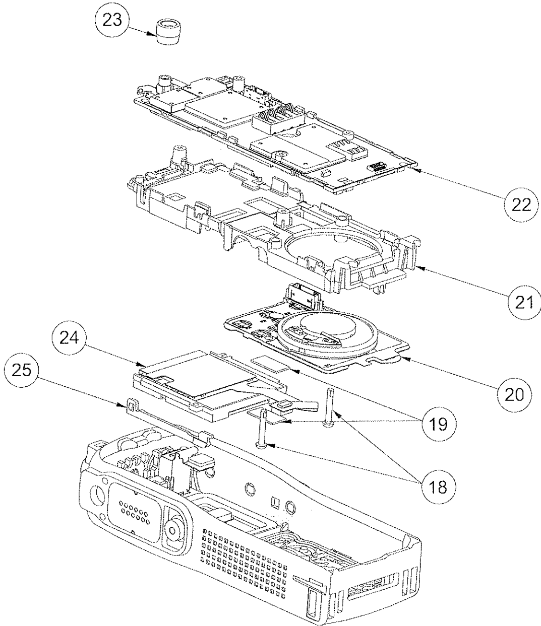
Figure 26 MTP850 S and MTP850 FuG — Exploded View 2
