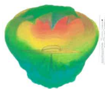
3D Gain Plot Top (3600MHz)
