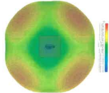
3D Gain Plot Side (2100MHz)
